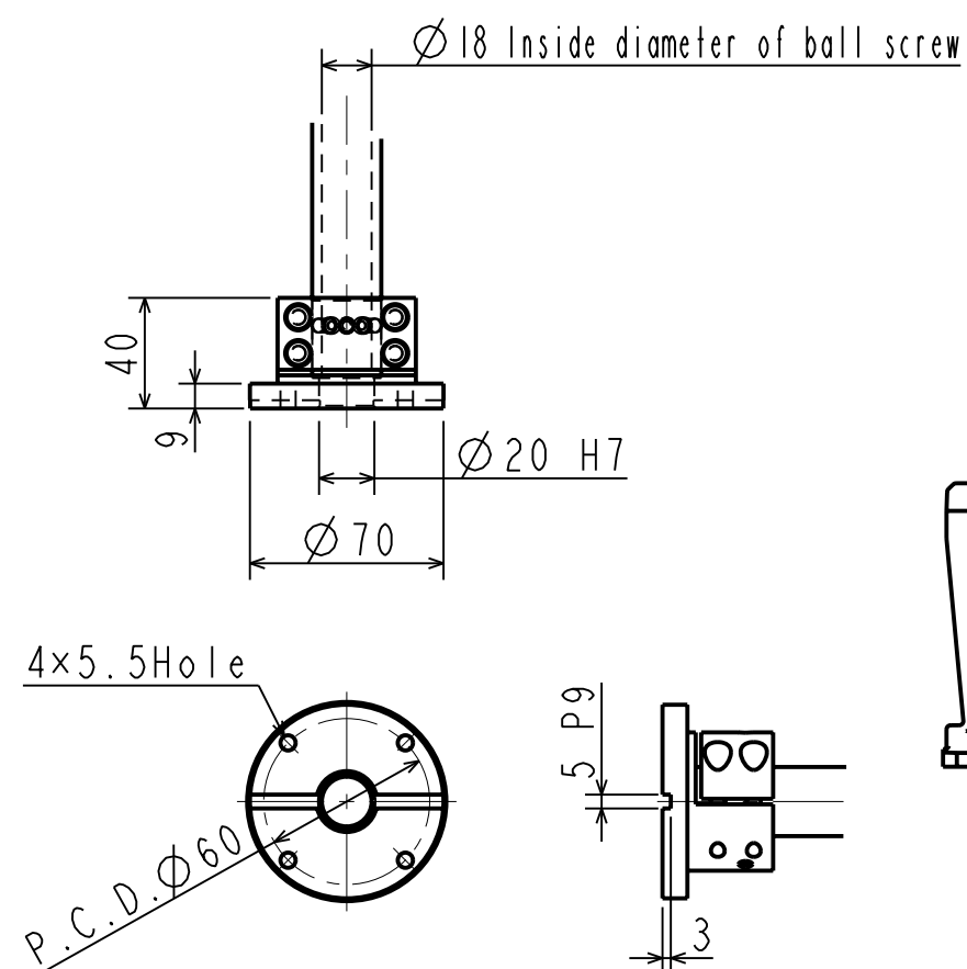
Detail of hand fixture scale 1:3
