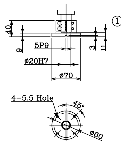
Part A detail(End-effector mount)
