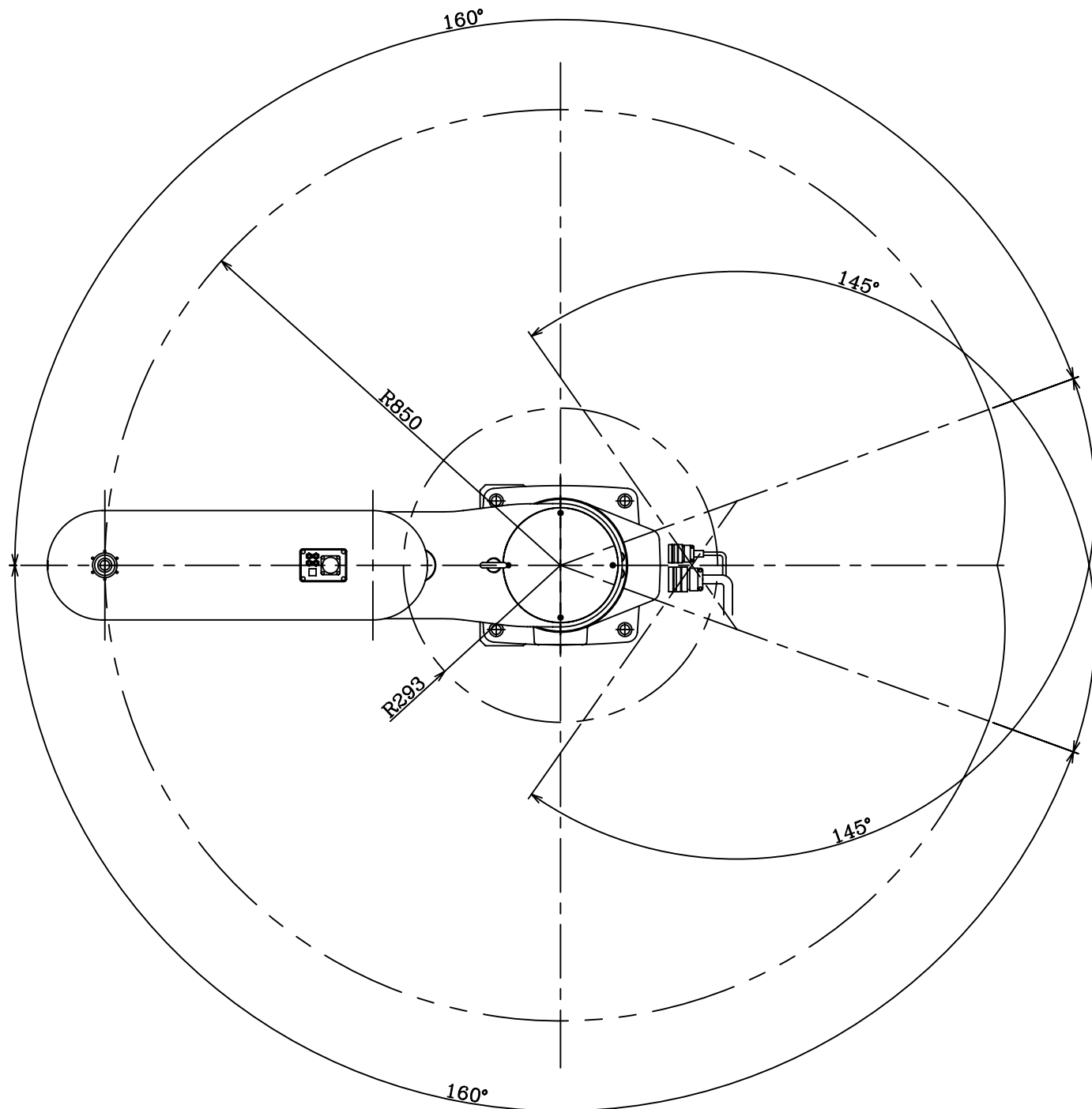
Part A; Working envelope
